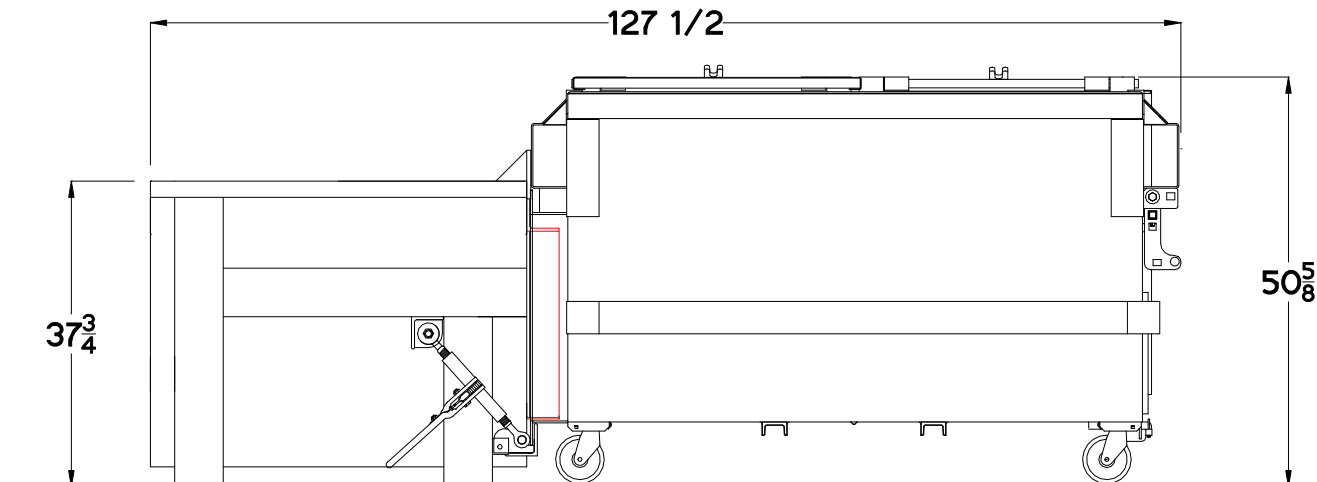
SIDE ELEVATION
