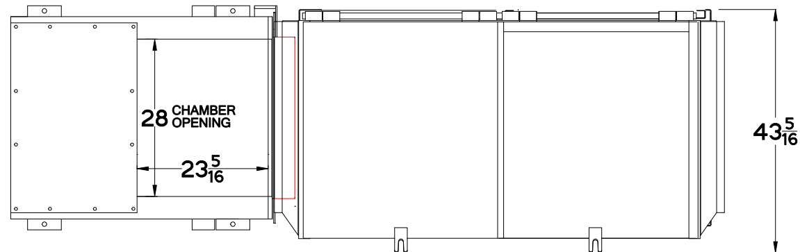
SIDE ELEVATION
