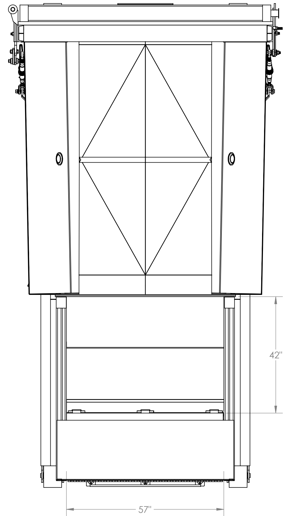
CHARGE CHAMBER DIMENSIONS
